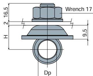
Tightening eyebolt (with nut)
